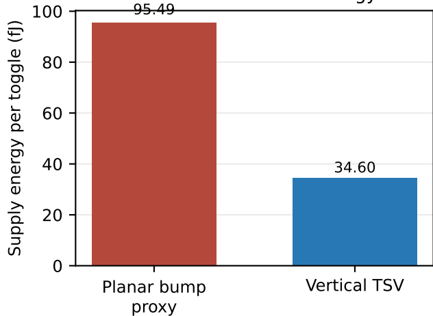
Transistor-level link energy
