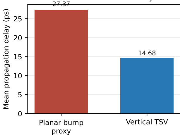
Transistor-level link delay
