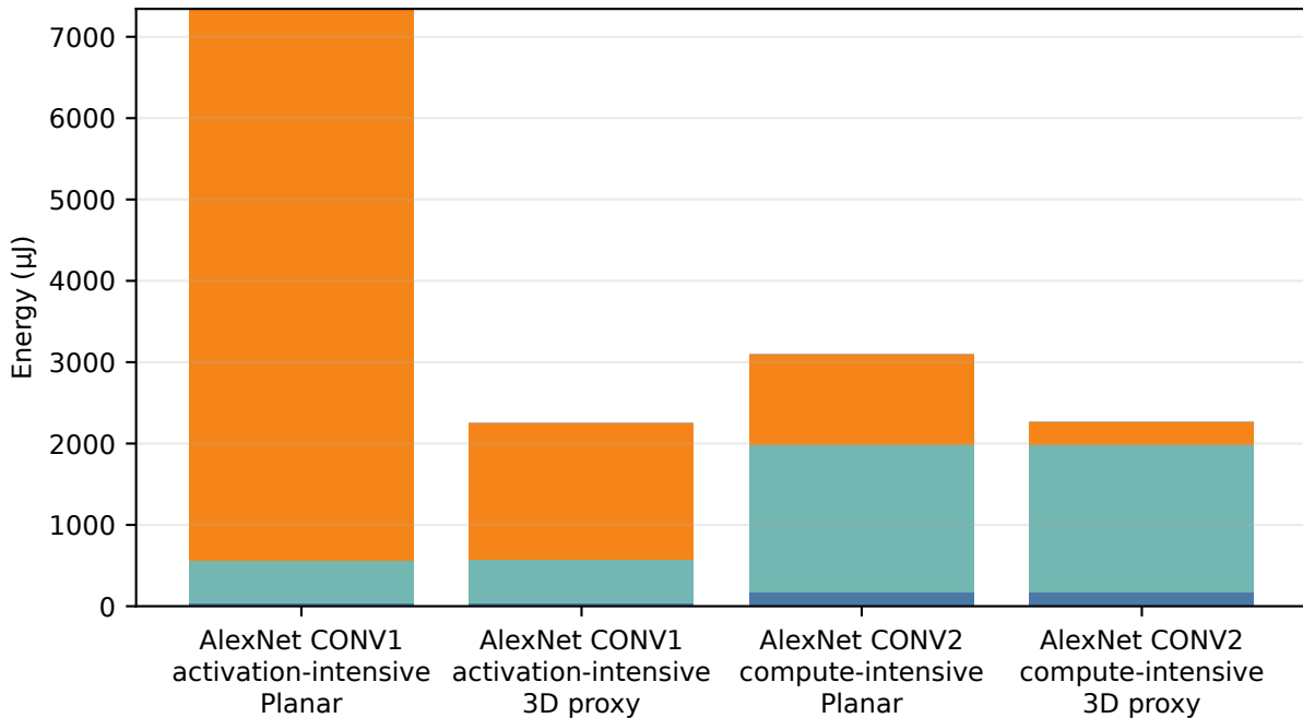
Timeloop/Accelergy energy breakdown Compute On-chip buffers DRAM / stacked SRAM Other/rounding
