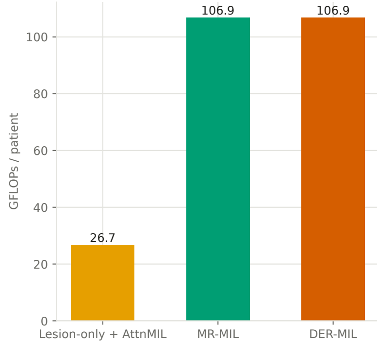
(b) Inference FLOPs, 3-frame bag (measured, torch.profiler)
