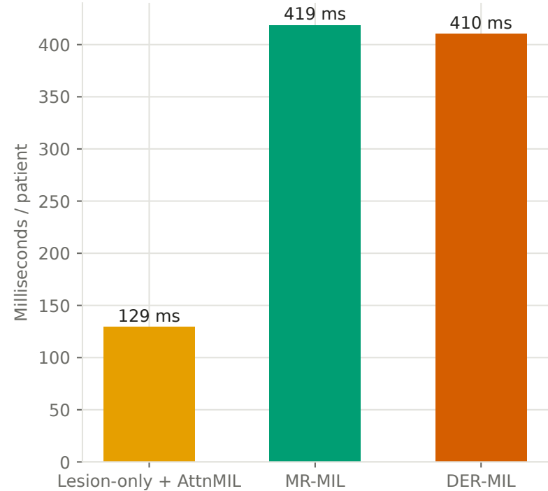
(c) CPU inference latency, 3-frame bag (measured on this machine, 20-run mean)
