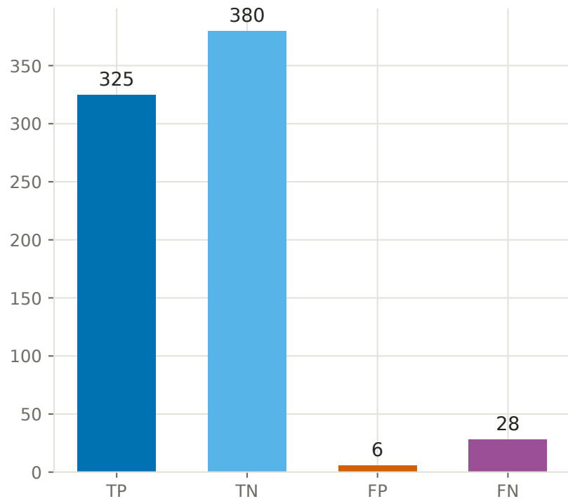
(a) Outcome counts, threshold 0.5 ConvNeXt-Tiny, ThyroidXL test, n=739
