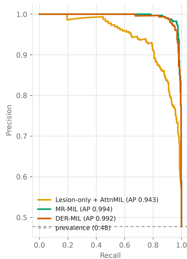
(b) Precision-recall -- ThyroidXL test
