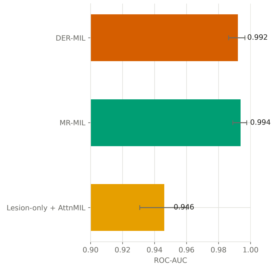
(c) ROC-AUC, 95% bootstrap CI
