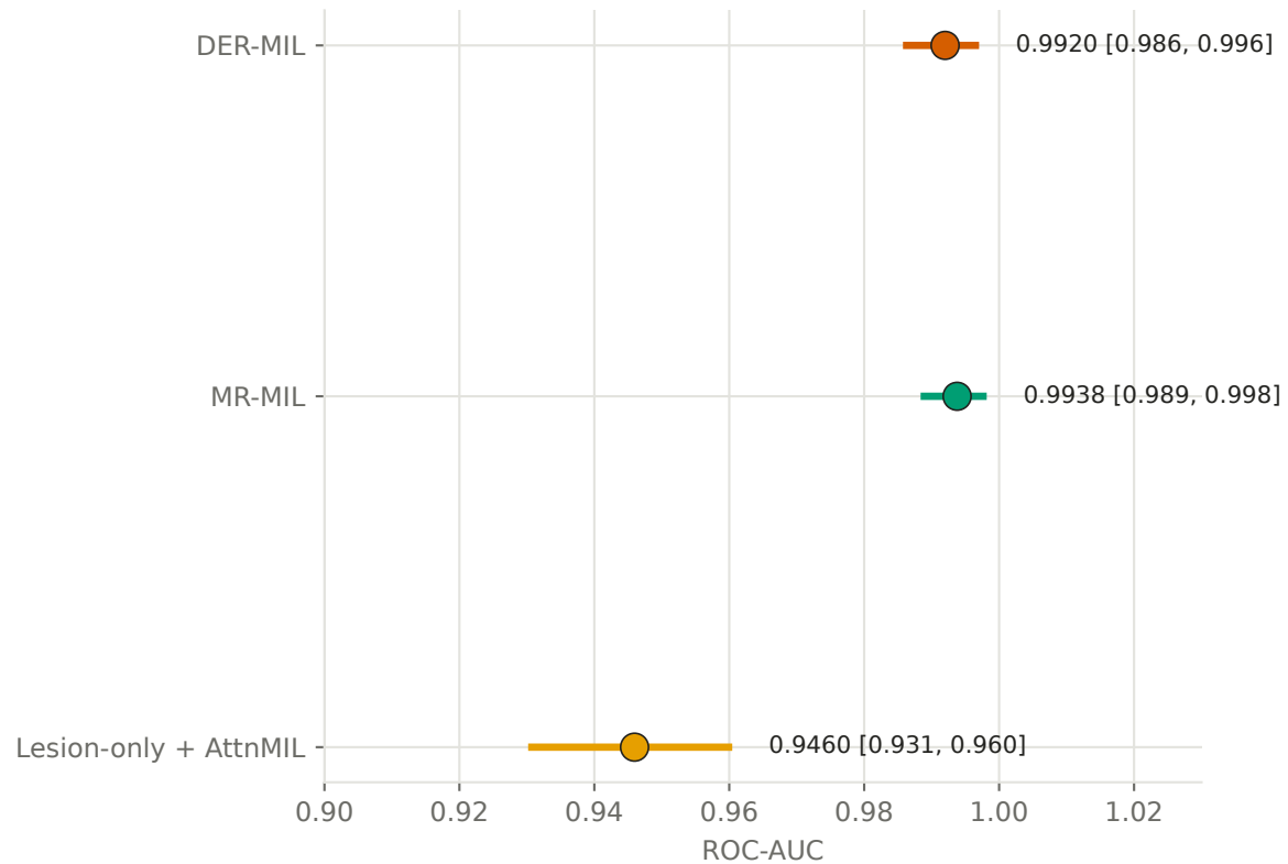
(b) Test-set ROC-AUC, 95%% bootstrap CI ConvNeXt-Tiny (2000 resamples, n=739)
