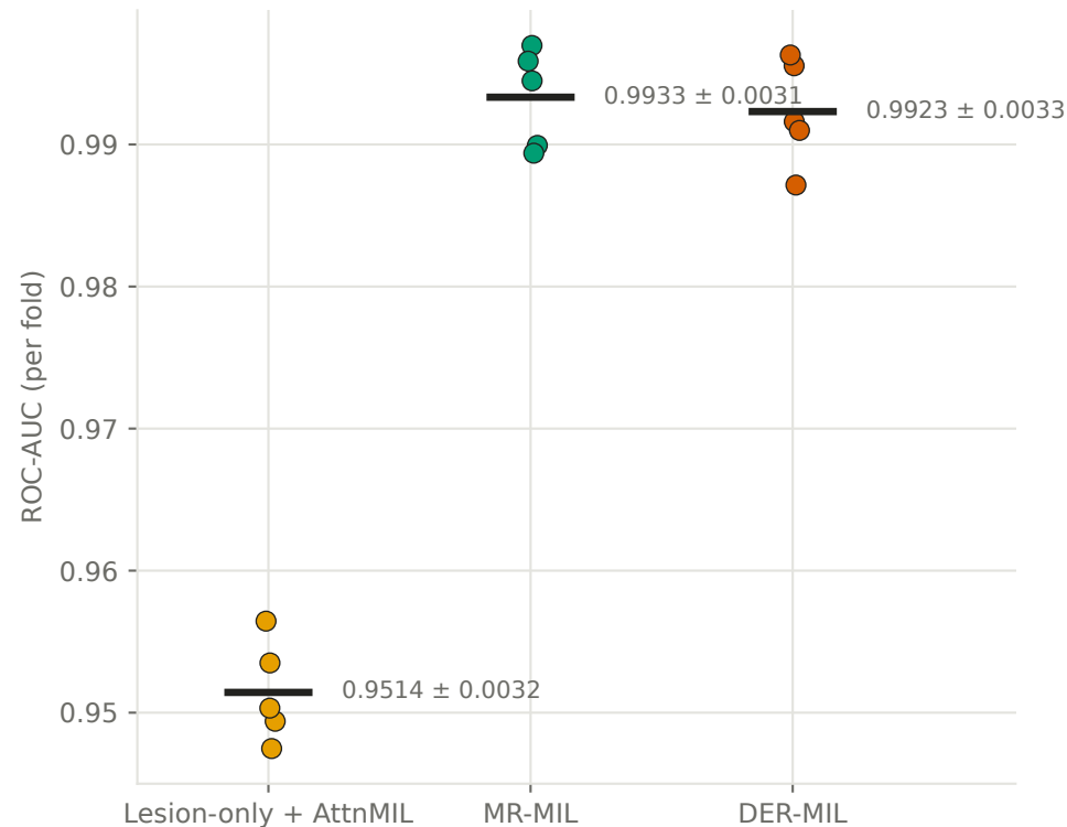
(a) 5-fold out-of-fold ROC-AUC, ConvNeXt-Tiny ThyroidXL development cohort, n=3354
