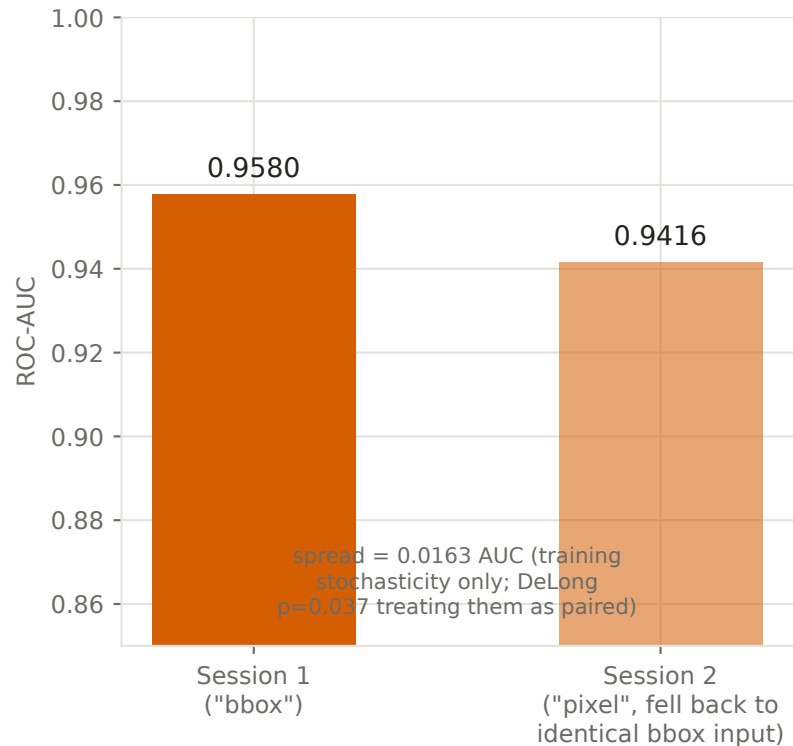
(b) Two runs, identical config & input (TN5000 ships 0 pixel masks of 5000)
