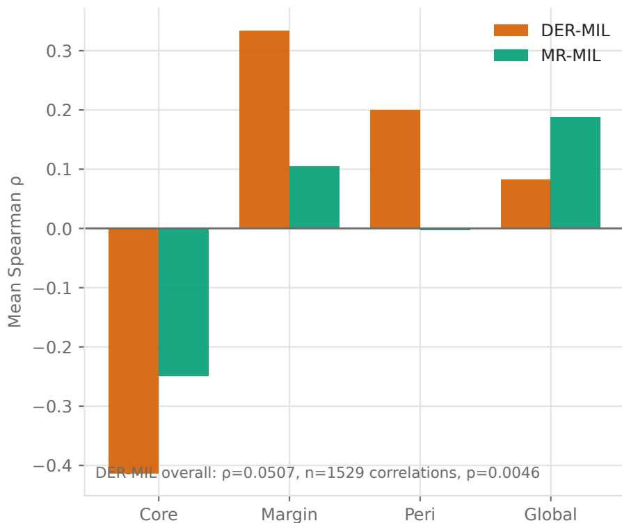
(c) Reliability predicts influence? Within-patient Spearman \rho , R vs |\Delta p| (across frames)
