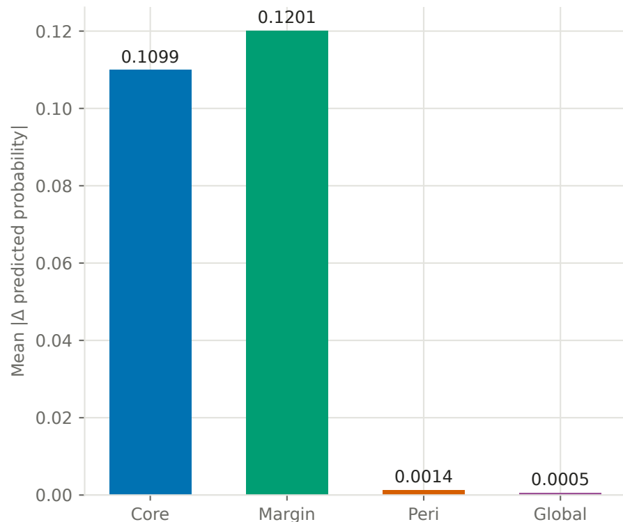
(a) Counterfactual influence by region (mean |\Delta p| when suppressed, DER-MIL)
