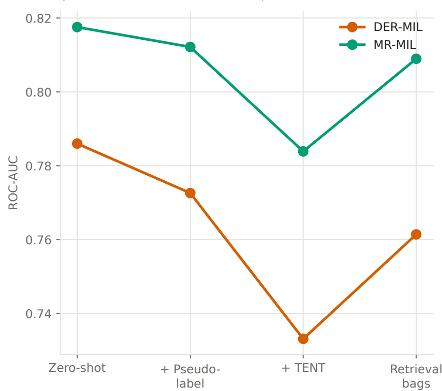
(b) Label-free adaptation arms (no TN5000 label ever used)
