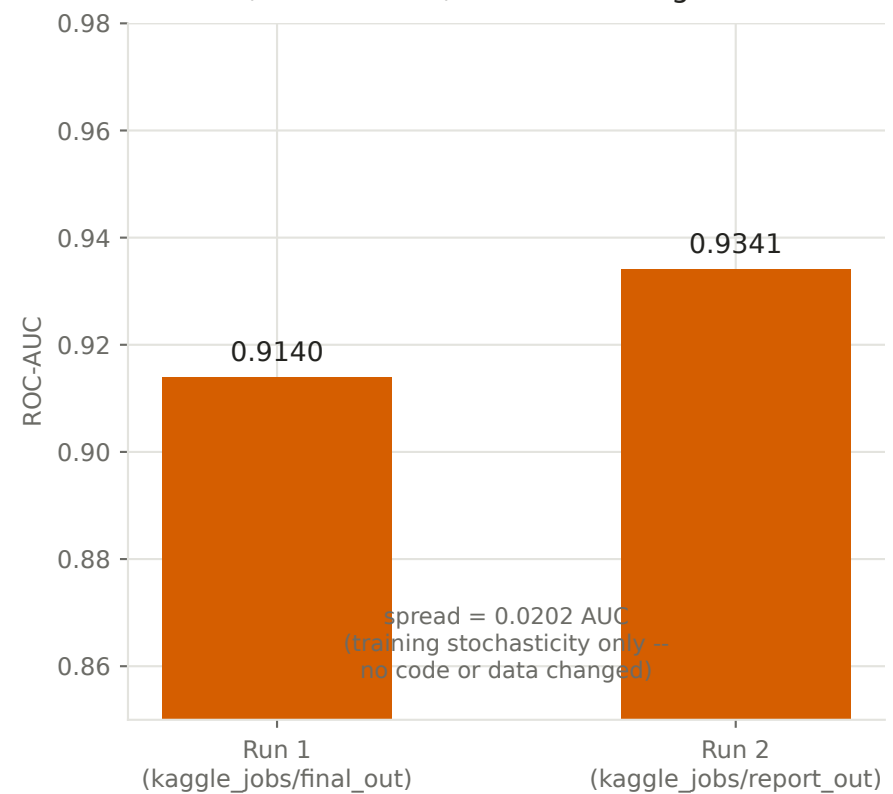
(c) Identical config, two sessions DER-MIL, bbox masks, same 250 images
