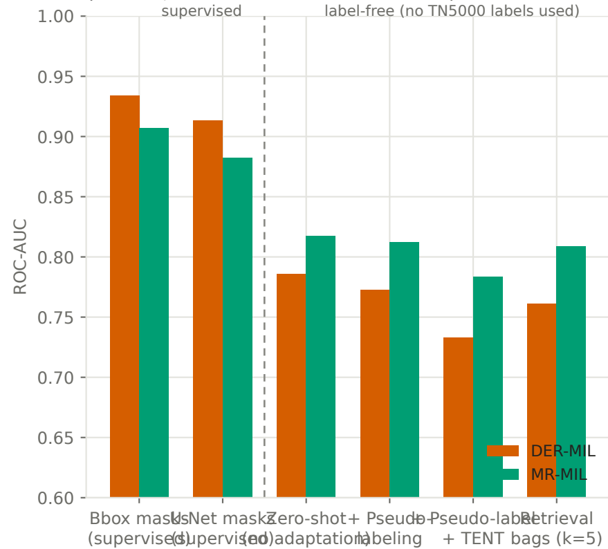
(a) TN5000 adaptation-arm ladder, ResNet-50 (n=250, class-balanced eval subset)
