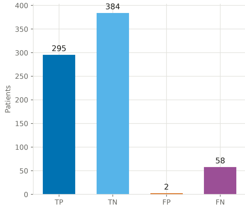
(a) Outcome counts, threshold 0.5 ThyroidXL test, n=739
