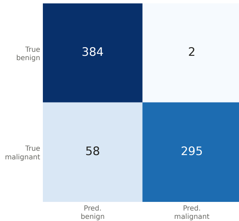
(f) DER-MIL
