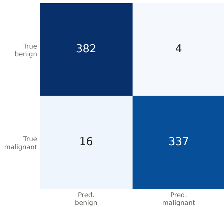
(e) MR-MIL
