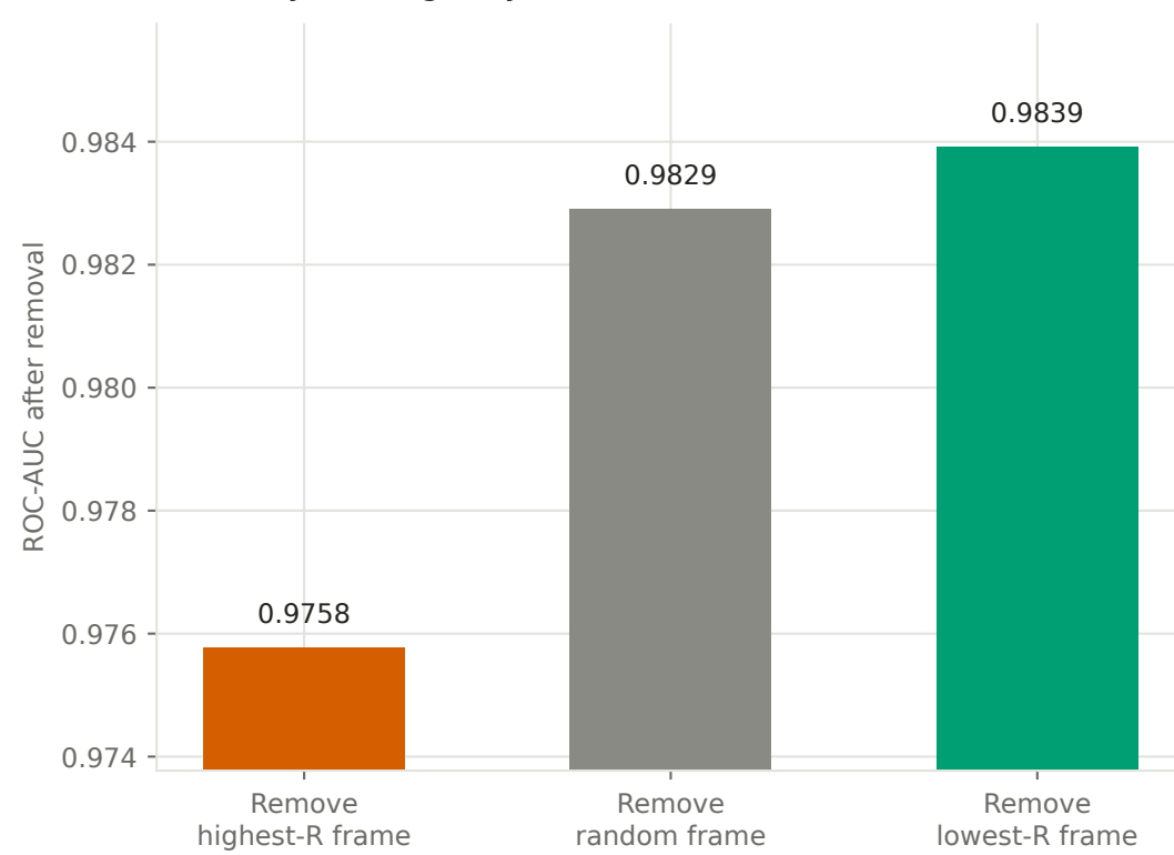
(b) One frame removed, by DER-MIL's own reliability ranking (ThyroidXL test)
