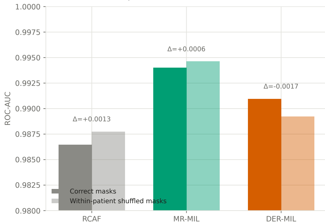
(c) Within-patient mask-identity shuffle (shortcut-reliance probe)
