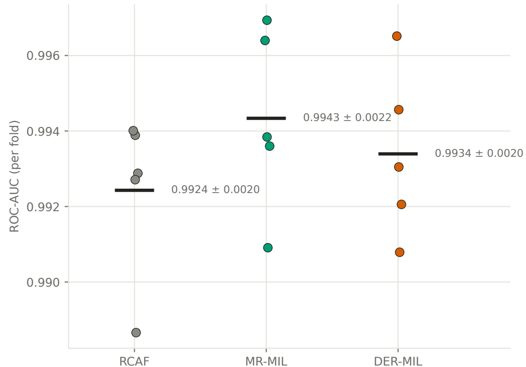
(a) 5-fold out-of-fold ROC-AUC ThyroidXL development cohort, n=3354
