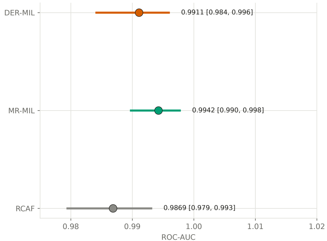
(b) Test-set ROC-AUC, 95% bootstrap CI (2000 resamples, n=739)
