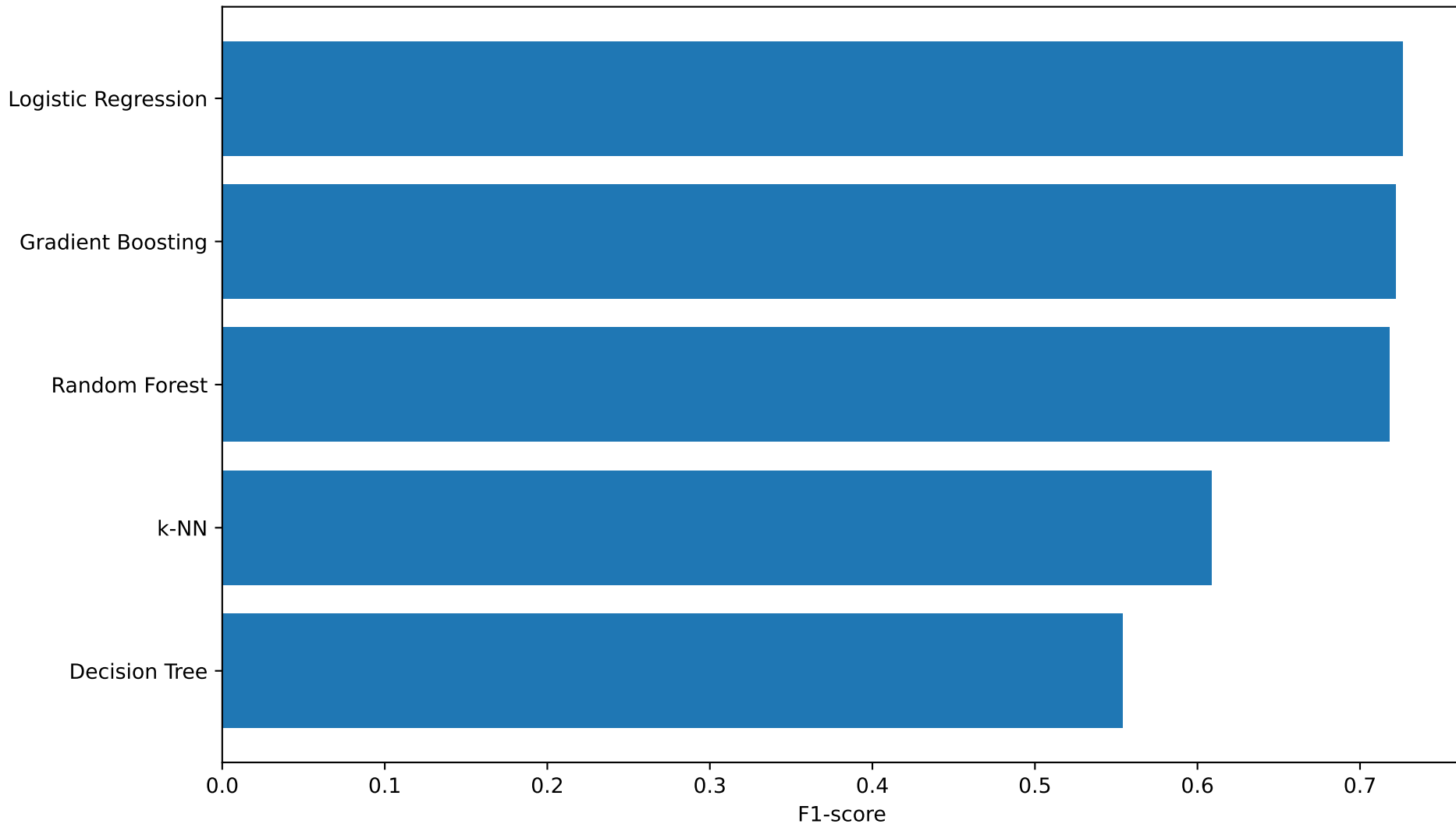
RQ2: Candidate Model Ranking by F1-score
