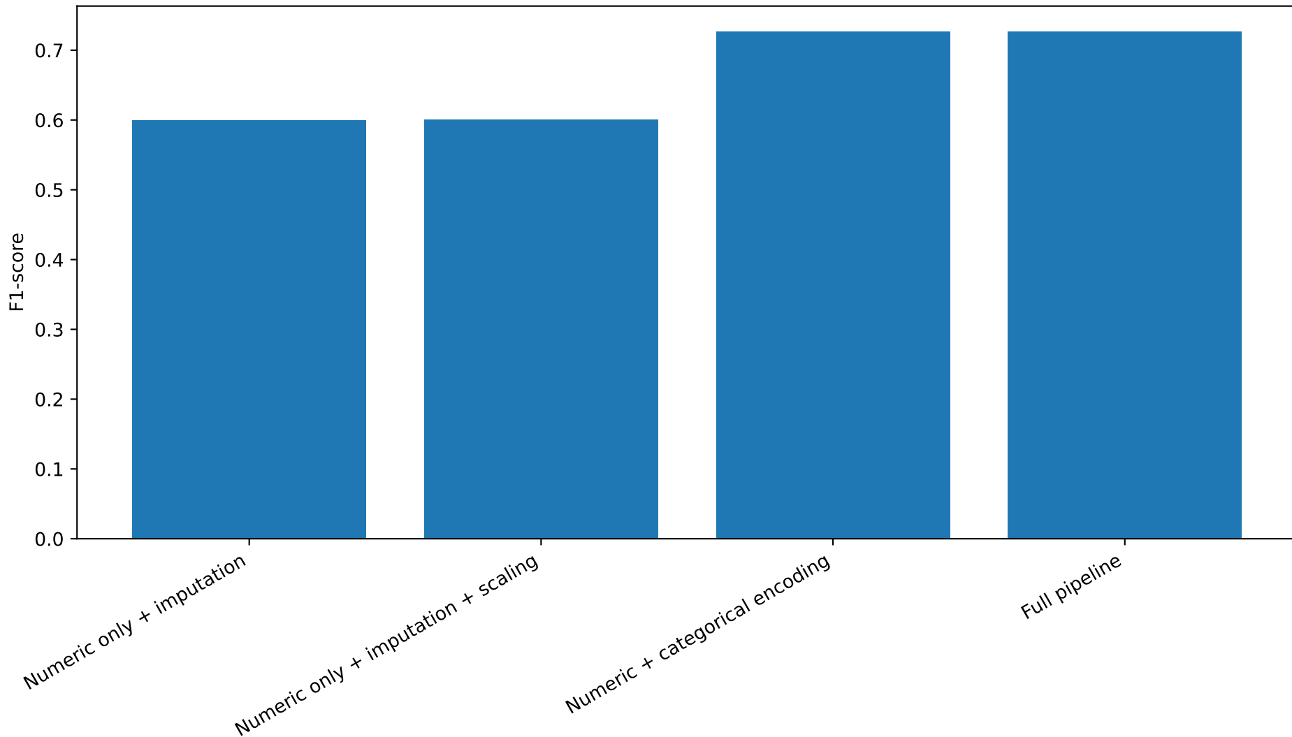
RQ3: Impact of Preprocessing on Logistic Regression
