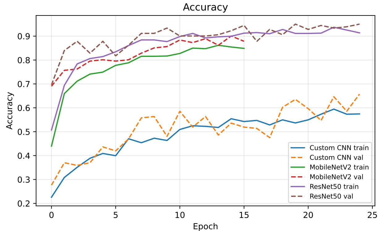
Figure 3 - Training and validation curves
