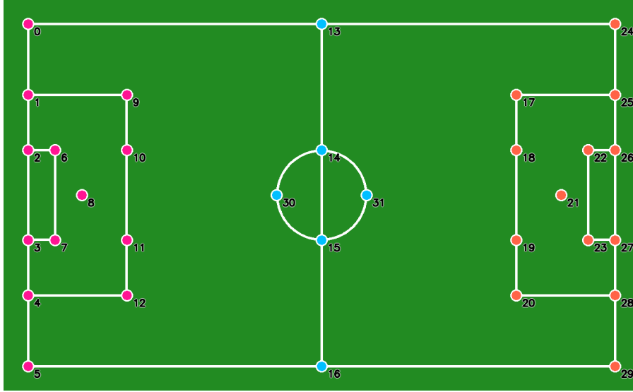
Figure 3.6: Pitch-keypoint template used for registration. The 32 landmarks correspond to stable pitch-line intersections, penalty-area corners, halfway-line points, and centre-circle points with known pitch-space coordinates. The fixed correspondence between detected image-space keypoints and this pitch-space template supplies the point pairs used by the DLT homography estimator.
