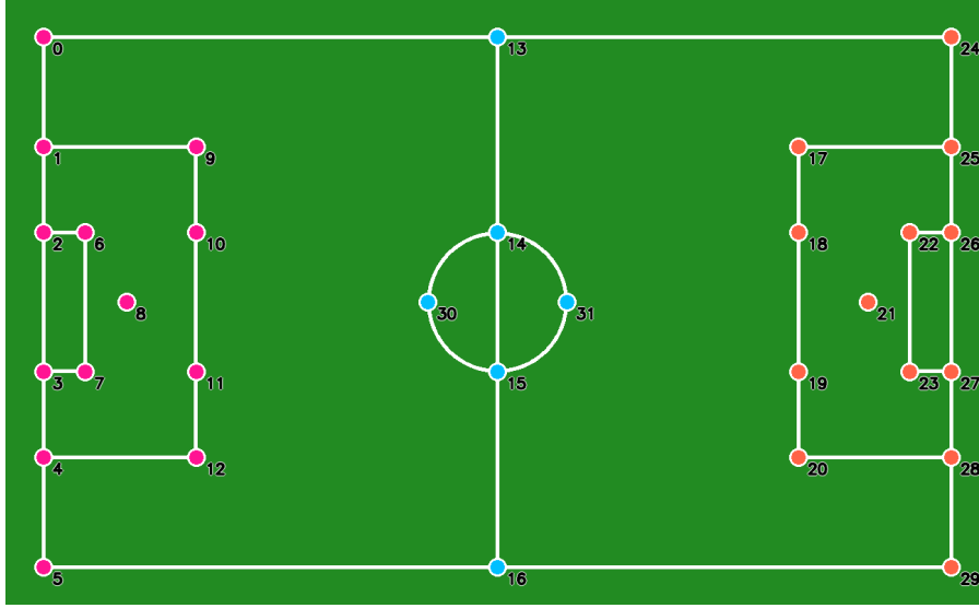
Figure 3.5: Pitch-keypoint template used for registration. The 32 landmarks correspond to stable pitch-line intersections, penalty-area corners, halfway-line points, and centre-circle points with known pitch-space coordinates. The fixed correspondence between detected image-space keypoints and this pitch-space template supplies the point pairs used by the DLT homography estimator.
