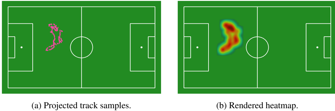
Figure 3.8: Per-track heatmap construction. Projected pitch-space positions are accumulated in a track-specific occupancy grid and rendered with smoothing and \gamma correction for visual readability.
