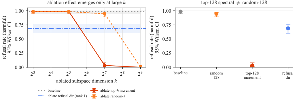
Figure 10: Causal ablation of the o_proj increment subspace (95% Wilson intervals). Left : rightward removes more directions; lower means stronger refusal suppression. Red is the damaging spectral ablation, orange a same-dimensional random control, and blue the rank-one positive control. Right : at k=128 , spectral ablation reaches 3.1% refusal versus 94.5% for random ablation. This intervention also harms capability.
