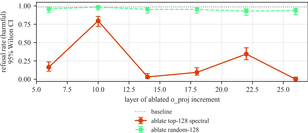
spectral subspace is ablation-sensitive at tested layers
