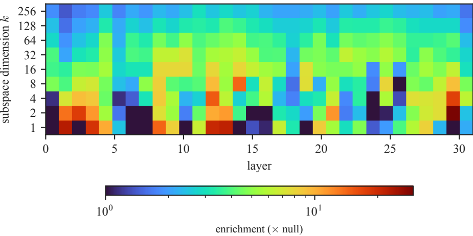
Refusal-direction enrichment over null (o_proj increment)
