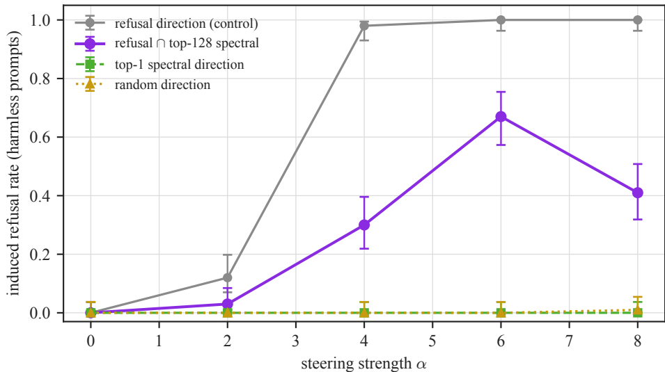
steering along the spectral subspace induces refusal
