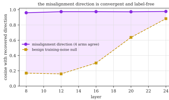
Figure 11: The misalignment direction is convergent across all layers (mean cosine of the four per-seed directions with the seed-averaged direction, 0.96 to 0.98), but cleanly separated from benign training noise only in the early-middle layers: the benign-versus-benign null is 0.16 at layer 12 and climbs to 0.88 by layer 24. The shaded gap is the separable signal.
