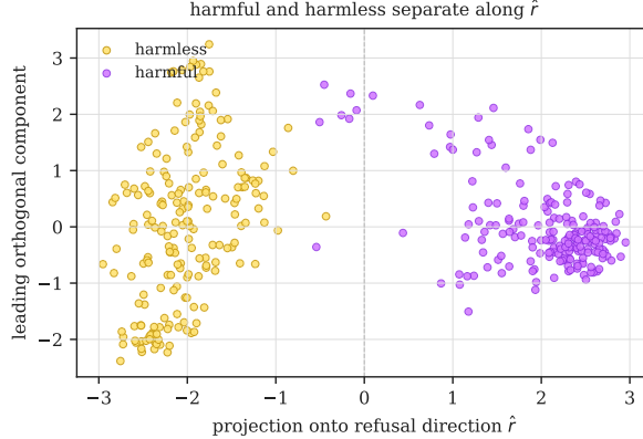
Figure 5: Last-token residual activations at layer 14 for harmful and harmless prompts, projected onto the refusal direction \hat{r} (horizontal) and the leading orthogonal component (vertical). The two classes separate along \hat{r} alone, which is the direction we then locate in the increment’s spectrum.
