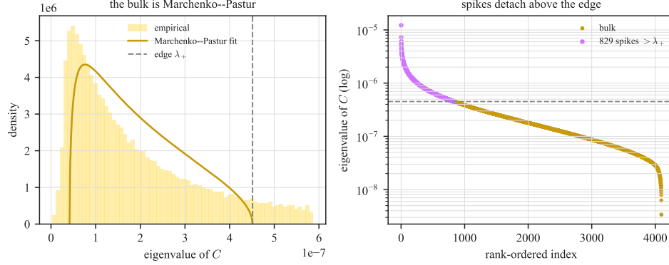
Figure 3: Spectrum of the alignment increment for a representative matrix ( gate_proj , layer 15; all 4096 eigenvalues of C ). Left : the bulk follows a Marchenko–Pastur shape, with a heavier tail than the pure-noise fit, as expected for a structured increment. Right : 829 eigenvalues lie above the raw Baik–Ben Arous–Péché edge \lambda_+ (821 clear the conservative six-Tracy–Widom counting threshold), the top one at 27\times the edge. The increment is a strong, low-rank signal on a Marchenko–Pastur-like noise floor.
