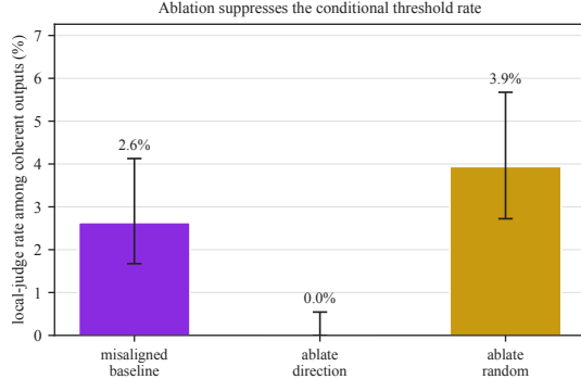
Figure 16: Ablation sensitivity of the recovered in-sample direction, with 95% Wilson intervals. The intervened arm contributed to the pooled direction. Ablating it from that misaligned arm drives the local-judge threshold rate from 2.6% (18/683) to 0.0% (0/702), while ablating a random direction of equal dimension leaves it at 3.9% (27/685). Across all 800 outputs per condition, the joint misalignment-and-coherence rates are 2.3%, 0.0%, and 3.4%. Low-strength addition to a benign arm increases measured misalignment, whereas increasing the strength primarily reduces coherence (reported in the text and summarized in Figure 18).
