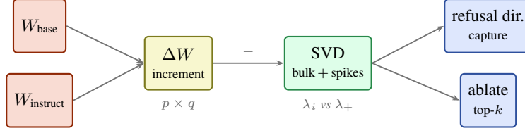
Figure 1: The refusal-analysis pipeline, read left to right. We difference the matched base and instruct checkpoints to form the post-training delta \Delta W , compare each SVD spectrum to a fitted Marchenko–Pastur reference, identify outlying singular directions, and test the leading spectral directions against the empirical refusal direction by both subspace capture and residual-stream projection.
