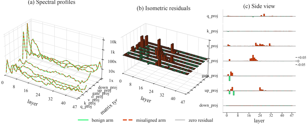
Figure 11: Matched 14B scalar scout across 48 layers and seven matrix types (336 matrices). (a) Top-eigenvalue-to-fitted-MP-edge profiles for the misaligned and benign-matched increments; height is logarithmic, so each decade is a tenfold increase. (b) An isometric view of the paired log-ratio \log_{10}(\text{misaligned}/\text{benign}) . (c) The same residuals from the side, where red bars above zero indicate a larger ratio for the misaligned arm and green bars below zero indicate a larger ratio for its benign match. Residuals change sign across layers and maps rather than showing a uniform shift. Together with the nearly identical medians in the text, this shows why the tested scalar concentration summaries do not separate the matched arms and why the subsequent analysis turns to directional information.
