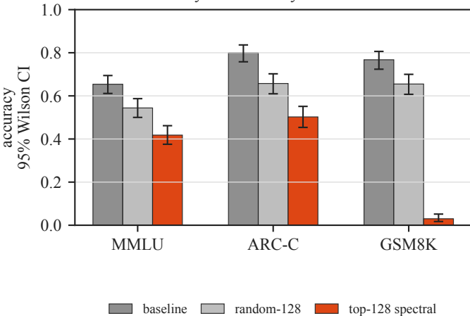
ordinary task accuracy under ablation
