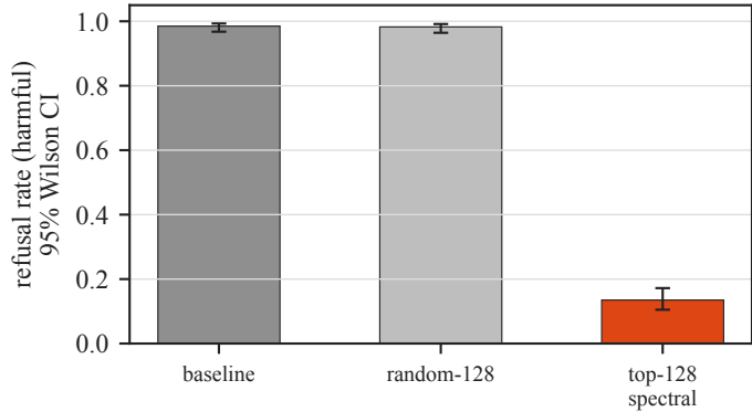
refusal rate under the same ablation
