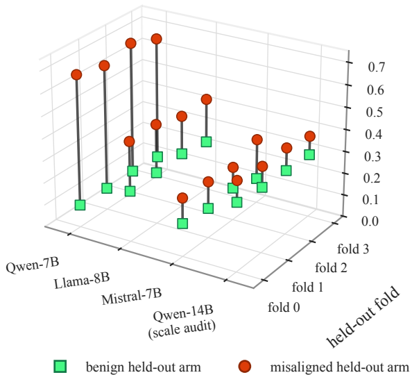
(a) Learned contrast direction
