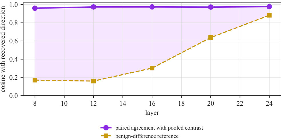
Internal agreement is largest in early-middle layers
