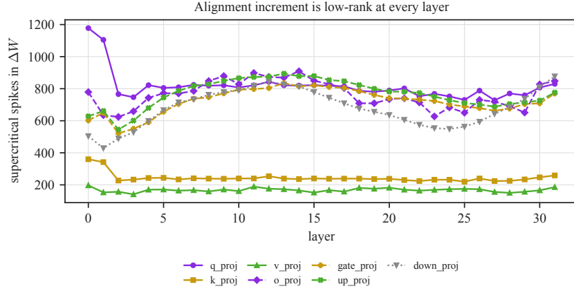
Figure 5: Supercritical spikes in \Delta W by layer and matrix type. Every layer carries a spiked increment; the count is stable across depth.
