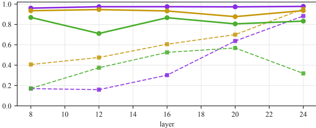
Direction converges across families in matched organism
