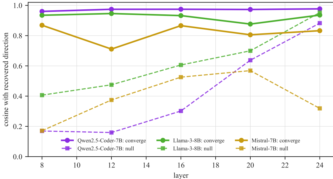
The misalignment direction converges across families
