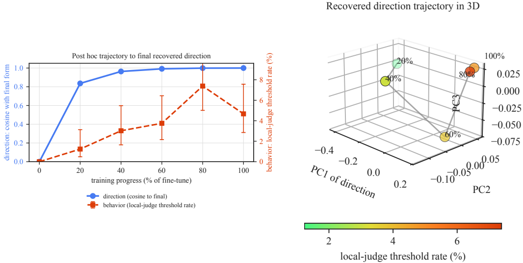
Figure 15: Retrospective trajectory. Left : rightward advances training; blue/red height is final-direction cosine/measured-misalignment rate. Cosine reaches 0.84 at 20% and 0.99 by 60%; the rate peaks at 80%. Right : Three-dimensional visualization of the same directions in their top PCA coordinates. Labels and line give training order, color gives rate, and proximity means similarity; axis signs and orientation are arbitrary. Step 0 is the base model, and both views are retrospective.
