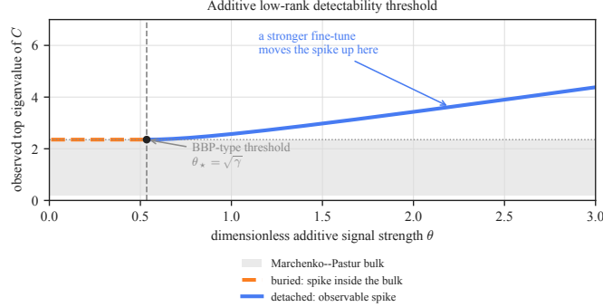
Figure 2: The rectangular additive spectral-visibility transition of Equation (1) (normalized \sigma^2 = 1 , at the representative aspect ratio \gamma \approx 0.29 of the feed-forward maps). Moving right increases planted-signal strength; moving up increases the observed top eigenvalue. Below \theta_* = \sqrt{\gamma} the signal remains buried at the noise edge; above it the detached branch rises and its singular vector acquires nonzero overlap with the planted direction.
