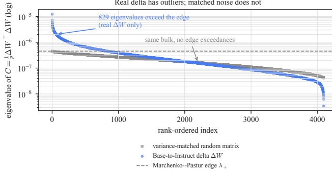
Figure 4: Ranked eigenvalues for the same increment (circle markers) and a variance-matched Gaussian matrix (square markers): left is larger, higher is stronger, and crossing the dashed edge marks visibility under the fitted reference. Both share the bulk, but only the real increment exceeds the edge. Matched fine-tunes provide the empirical control beyond this Gaussian reference.
