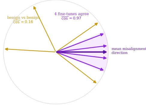
Figure 14: The recovered directions as geometry, drawn so that pairwise angles equal the measured cosines. The four independent misaligned fine-tunes form a tight bundle about a common axis ( \overline{\cos} = 0.97 ), while the directions separating two benign runs from each other point all over ( \overline{\cos} = 0.16 ). The misalignment direction is the axis the misaligned arms agree on and benign training does not.
