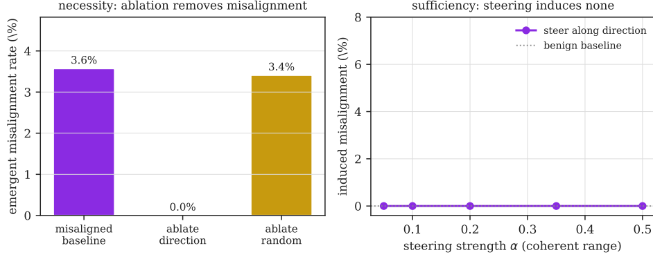
Figure 15: Causal tests of the recovered misalignment direction. Left (necessity) : ablating the direction from a misaligned arm drives emergent misalignment from 3.6% to 0%, while ablating a random direction of the same dimension leaves it at 3.4%. Right (sufficiency) : steering a benign arm along the direction, across the strength range that keeps generation coherent, induces no misalignment above the 0% baseline. The direction is necessary to remove the behavior but not sufficient to install it.
