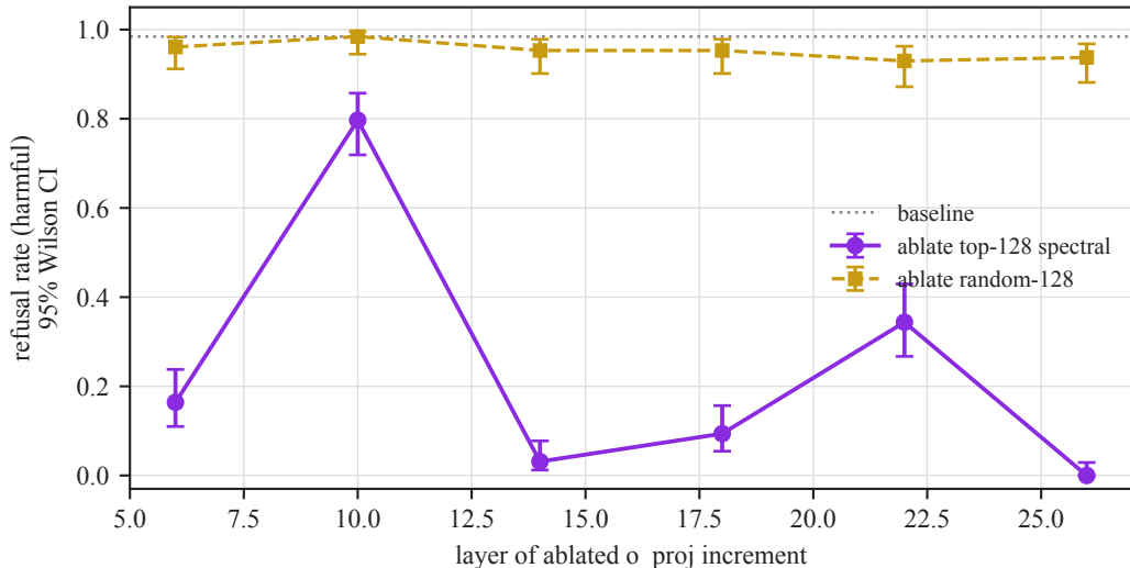
spectral subspace is ablation-sensitive at tested layers
