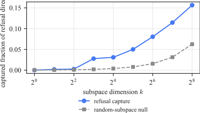
Refusal direction is enriched in top increment directions
