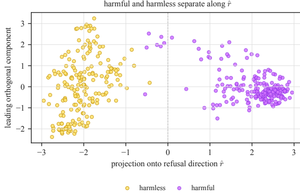
Figure 8: Last-token residual activations at layer 14 for harmful and harmless prompts, projected onto the refusal direction \hat{r} (horizontal) and the leading orthogonal component (vertical). The two classes separate primarily along \hat{r} ; the capture analysis below compares this axis with the increment’s singular subspaces.
