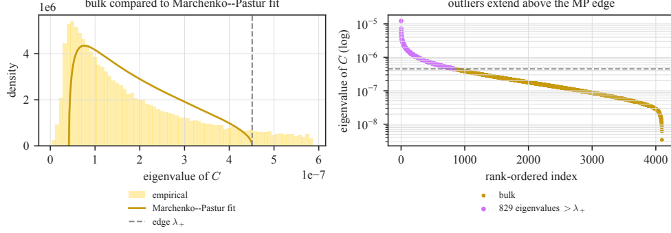
Figure 3: Spectrum of the Base-to-Instruct checkpoint delta for a representative matrix (gate_proj, layer 15; all 4096 eigenvalues of C ). Left : the bulk follows a Marchenko–Pastur shape, with a heavier tail than the pure-noise fit. Right : 829 eigenvalues lie above the MP upper edge \lambda_+ (821 clear the operational edge-plus-six-fluctuation-scale threshold), the top one at 27\times the edge. The refusal and misalignment interventions below test the behavioral relevance of these spectral components.
