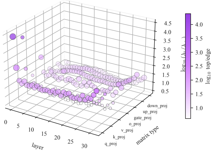
Figure 6: A three-dimensional view of the same full spectral sweep. Each point is one of the 224 layer-matrix increments; the height and color give the \log_{10} top-eigenvalue-to-edge ratio \lambda_1/\lambda_+ . The plot is a descriptive overview of where the strongest spiked structure appears across the alignment increment, not an alignment detector by itself.
