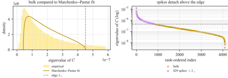
Figure 3: Spectrum of the alignment increment for a representative matrix (gate_proj, layer 15; all 4096 eigenvalues of C ). Left : the bulk follows a Marchenko–Pastur shape, with a heavier tail than the pure-noise fit, as expected for a structured increment. Right : 829 eigenvalues lie above the raw Baik–Ben Arous–Péché edge \lambda_+ (821 clear the conservative six-Tracy–Widom counting threshold), the top one at 27\times the edge. The increment is strongly concentrated relative to a Marchenko–Pastur-like visibility reference; this panel alone does not identify which part of the structure is alignment-relevant.
