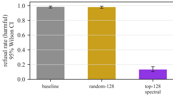
refusal rate under the same ablation
