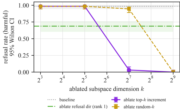
ablation effect emerges only at large k
