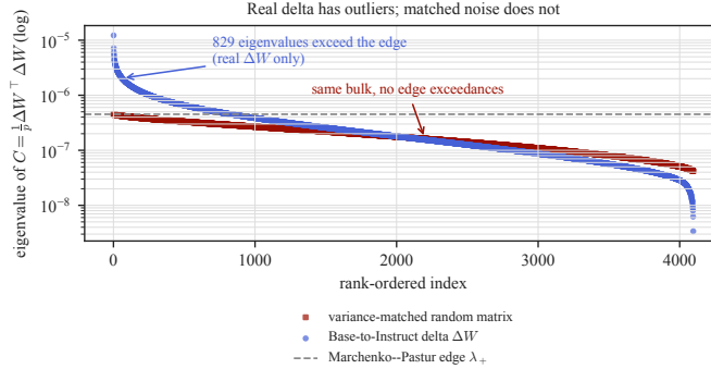
Figure 4: Ranked eigenvalues for the same increment (blue circles) and a variance-matched Gaussian matrix (red squares): left is larger, higher is stronger, and crossing the dashed edge marks MP visibility. Both share the bulk, but only the real increment detaches. Matched fine-tunes provide the empirical control beyond this Gaussian reference.
