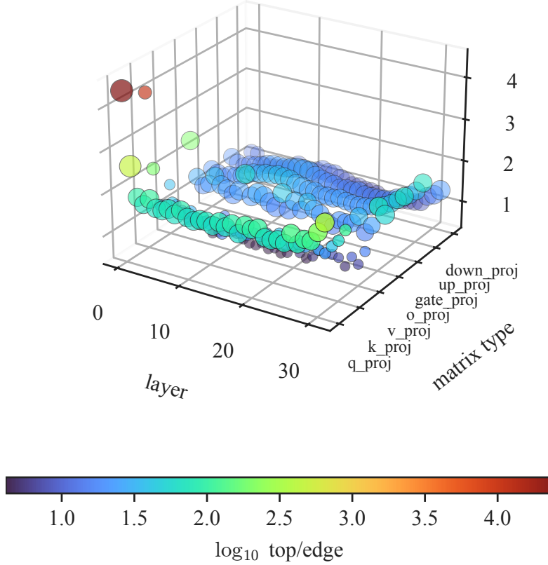
Figure 6: The full spectral sweep: the base plane locates each of the 224 layer–matrix increments, while height and color moving from violet toward red mean a larger \log_{10}(\lambda_1/\lambda_+) and thus greater separation above the fitted edge. MP-visible structure appears throughout the delta.
