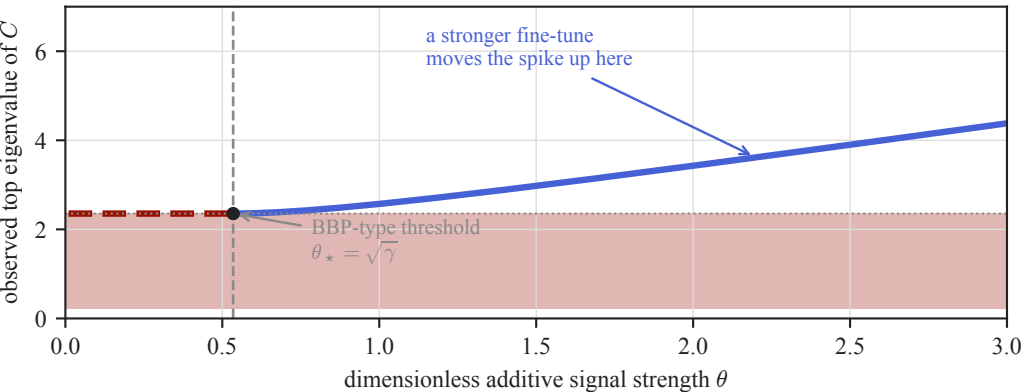
Additive low-rank detectability threshold
