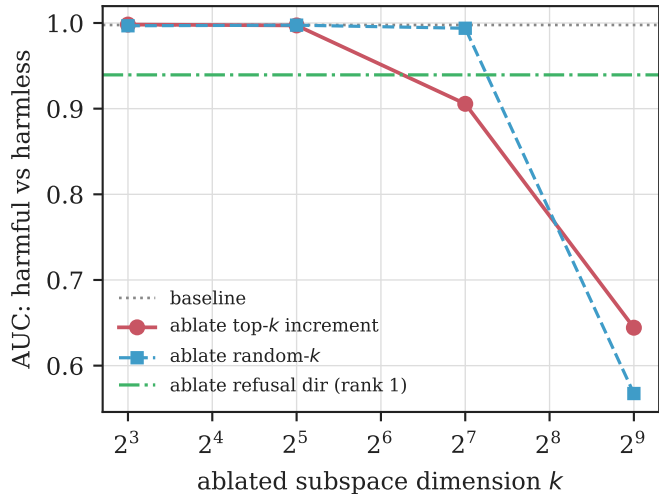
necessity emerges only at large k
