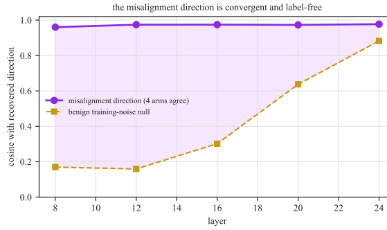
Figure 14: The misalignment direction is convergent across all layers (mean cosine of the four per-seed directions with the seed-averaged direction, 0.96 to 0.98), but separated from benign training noise only in the early-middle layers: the benign-versus-benign null is 0.16 at layer 12 and climbs to 0.88 by layer 24. The shaded gap is the separable signal.
