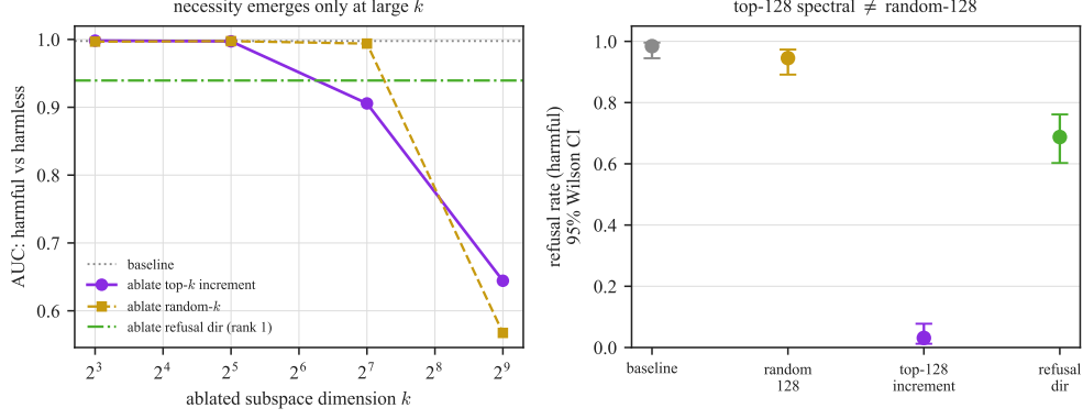
Figure 10: Causal ablation of the o_proj increment subspace. Left : harmful-versus-harmless separation (AUC) as the ablated dimension k grows, shown as a diagnostic because the committed artifact stores scalar AUCs rather than per-example scores for AUC intervals. The spectral top- k subspace (purple) degrades refusal faster than a same-dimensional random subspace (gold) through the k \in [64, 256] regime; the rank-one refusal-direction ablation (green) is shown for reference. Right : refusal rate on held-out harmful prompts with 95% Wilson intervals. Ablating the top-128 spectral directions collapses refusal to 3%, while a random 128-subspace leaves it at 94%, a clean dissociation with non-overlapping intervals.
