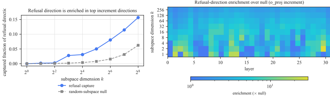
Figure 9: Left : captured fraction of the post-block-14 refusal direction by the top- k block-14 \text{o\_proj} increment subspace and the random reference. Rightward includes more directions; upward means more capture. Right : columns vary source block, rows vary k , and color gives enrichment over random.
