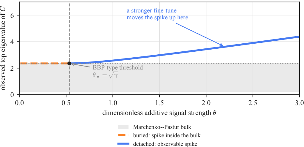
Rectangular additive spectral-visibility transition
