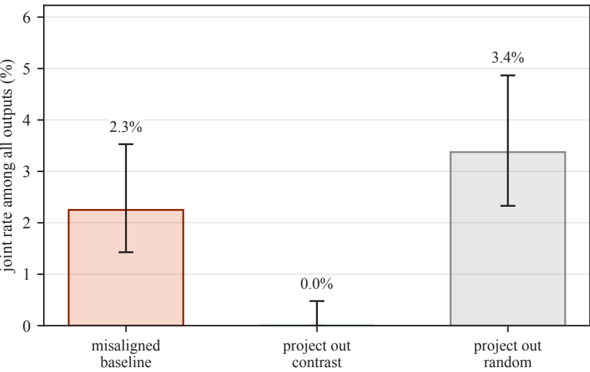
In-sample medical-contrast projection
