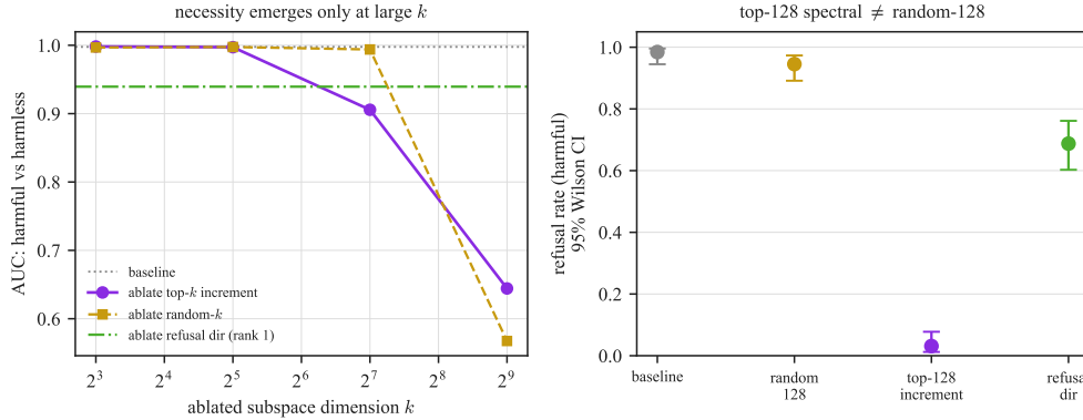
Figure 10: Causal ablation of the o_proj increment subspace. Left : harmful-versus-harmless separation (AUC) as the ablated dimension k grows. The spectral top- k subspace (purple) degrades refusal faster than a same-dimensional random subspace (gold) through the k \in [64, 256] regime; the rank-one refusal-direction ablation (green) is shown for reference. Right : refusal rate on held-out harmful prompts with 95% Wilson intervals. Ablating the top-128 spectral directions collapses refusal to 3%, while a random 128-subspace leaves it at 94%, a clean dissociation with non-overlapping intervals.
