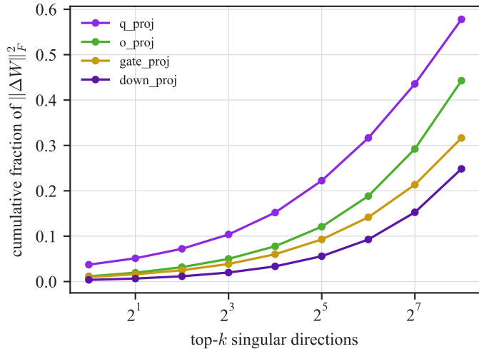
energy is front-loaded into a few directions
